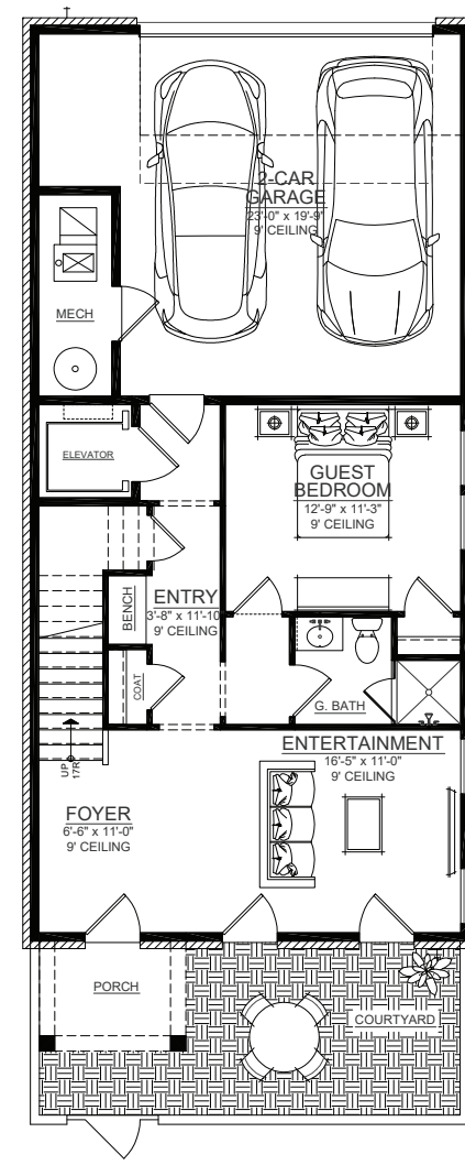
ALTERNATE TERRACE
