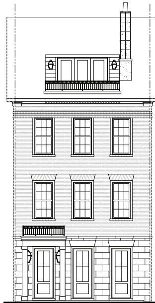
FRONT ELEVATION A
