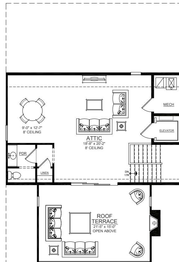
ATTIC
