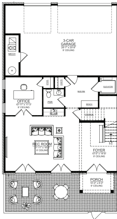
TERRACE
